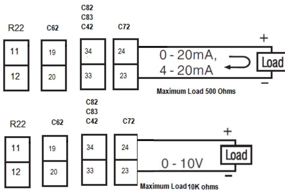
2-43 Retransmission Wiring
