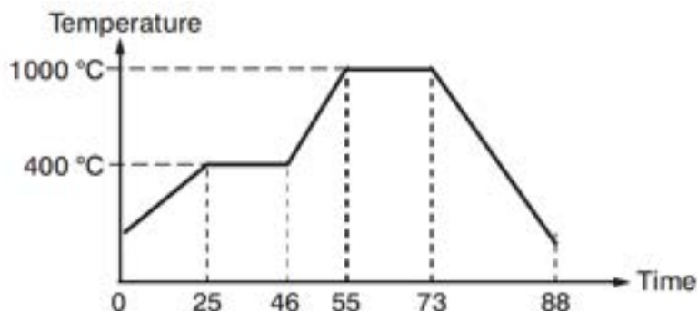
4-12 Temperature Profile of the Heat Treatment Chamber
