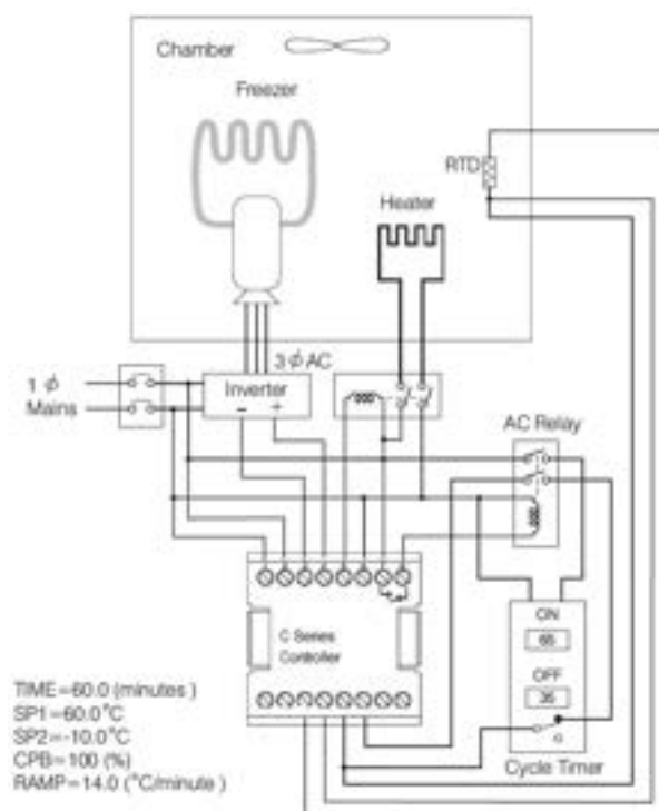
4-4 Ramp & Dwell Temperature Cycling Chamber
