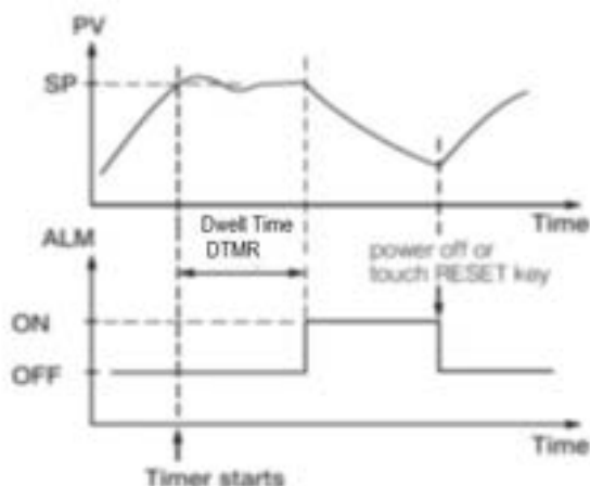
3-23 Dwell Timer
