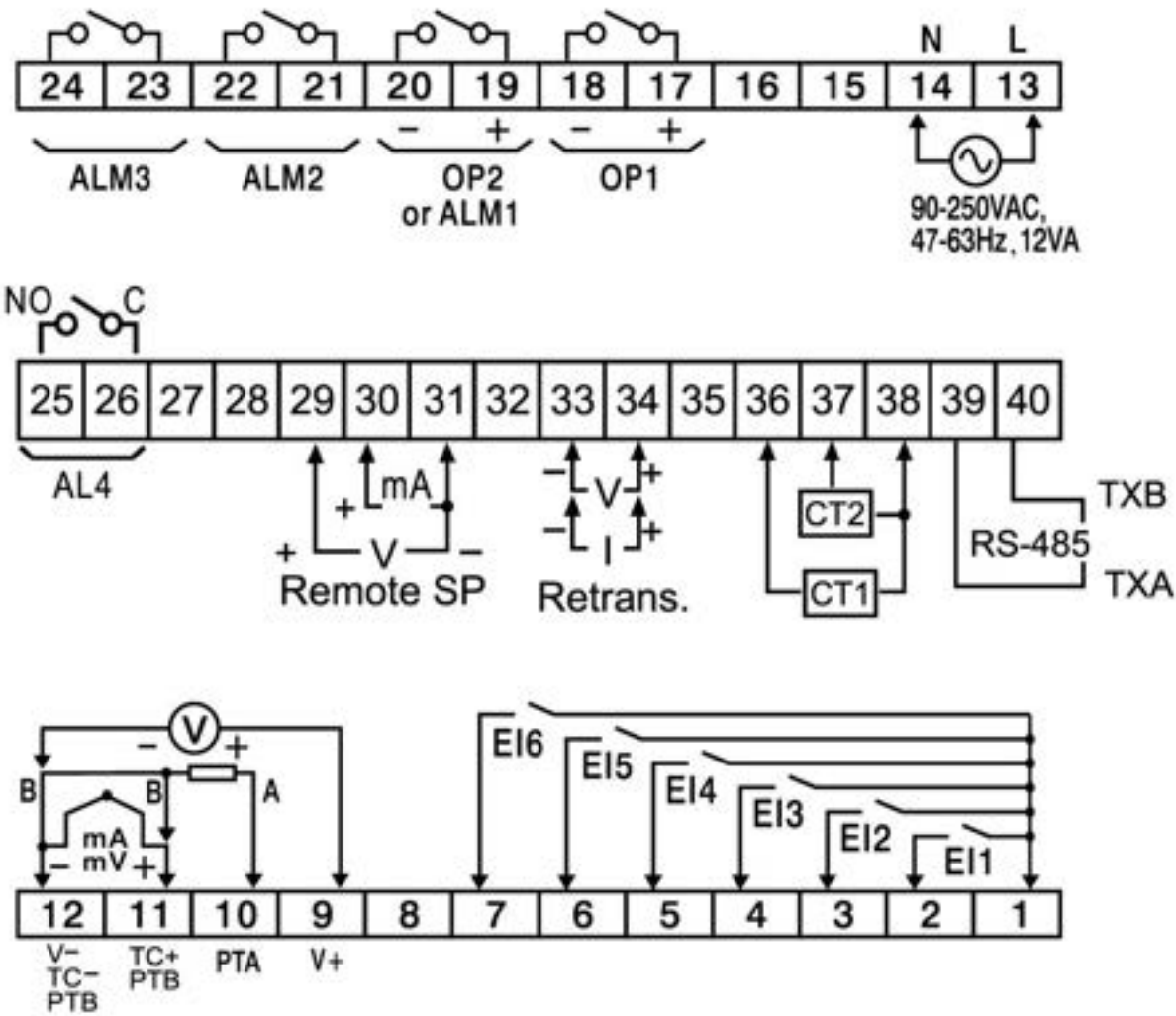
2-21 C83 Rear Terminal Connection
