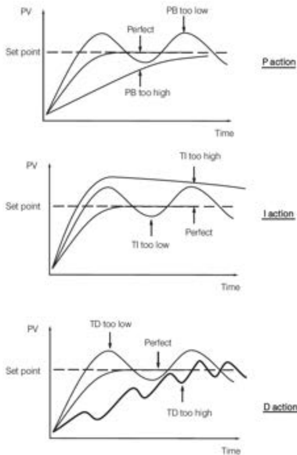
3-26 Effects of PID Adjustment
