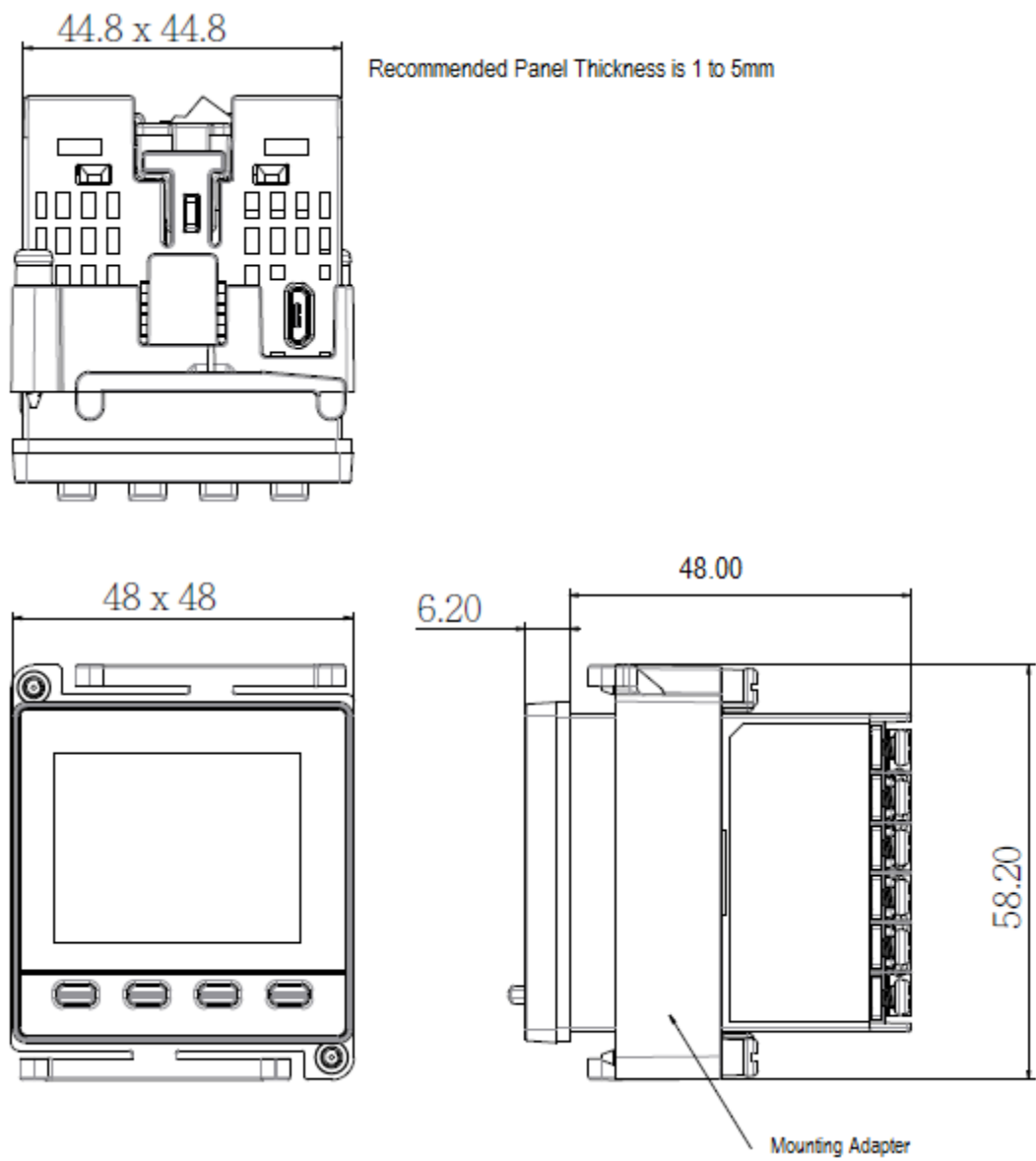
2-3 C62 Dimension with clamp
