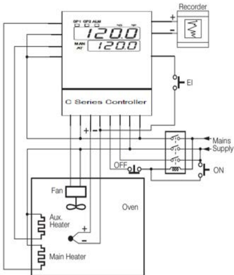
4-11 Heat Treatment Chamber
