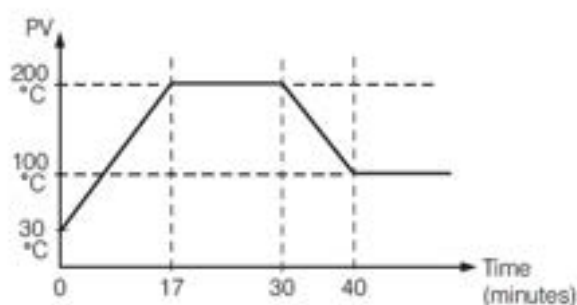
3-22 Ramp Function
