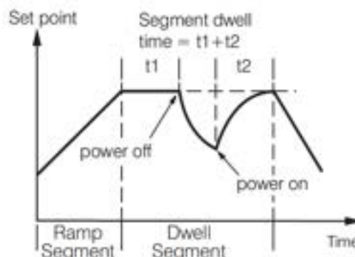
3-28 Power failure recovery from the profile at Dwell segment
