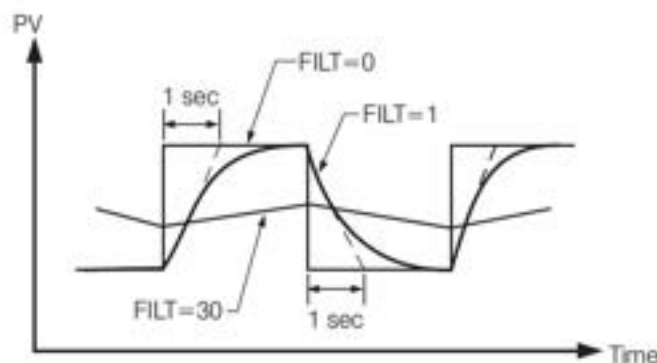
3-25 Filter Characteristics
