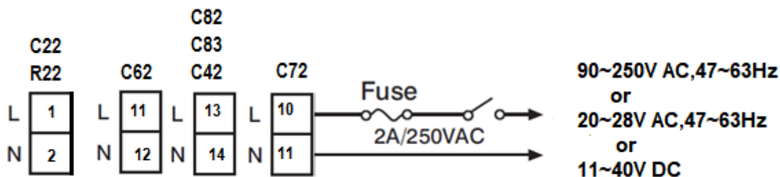
2-24 Power Wiring
