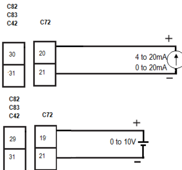
2-44 Remote SetPoint
