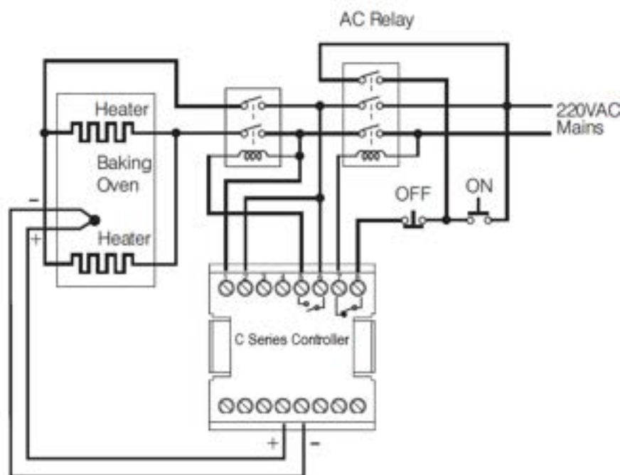
4-6 Bread Baking Oven
