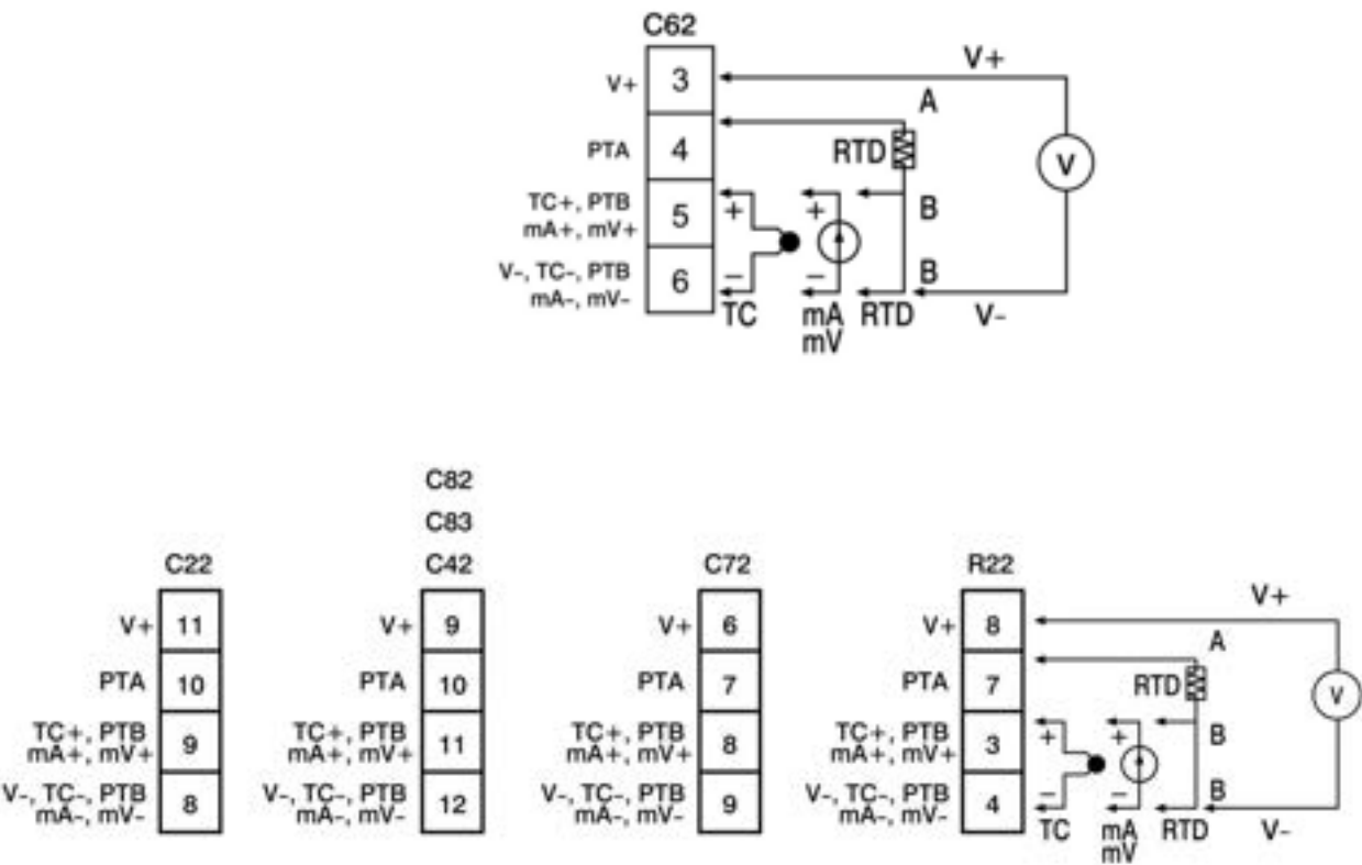
2-25 Sensor Input Wiring
