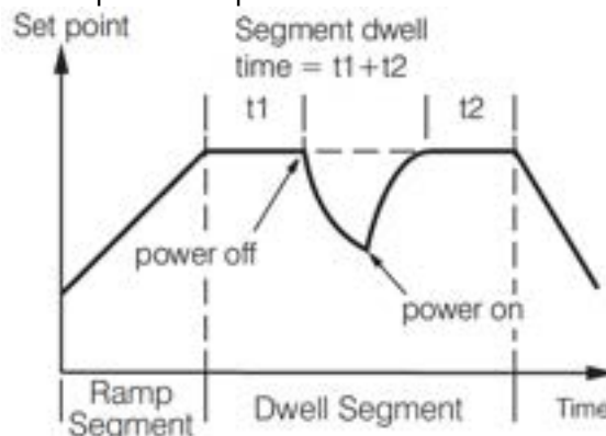
3-30 Power failure recovery from PV at Dwell segment
