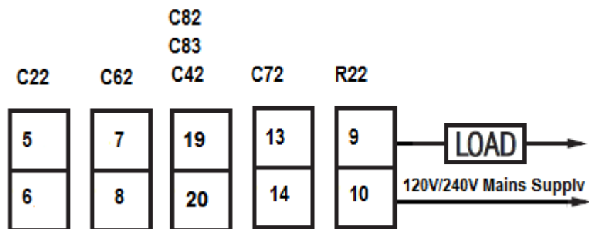
2-31 Output 2 Relay to Drive Load
