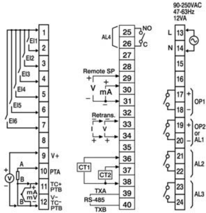
2-20 C82 & C42 Rear Terminal Connection
