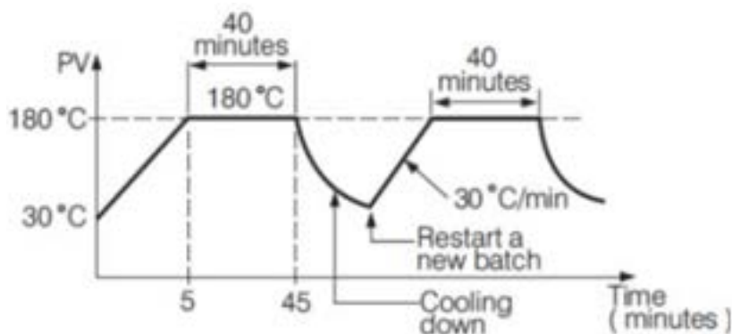
4-7 Temperature Profile of Baking Oven
