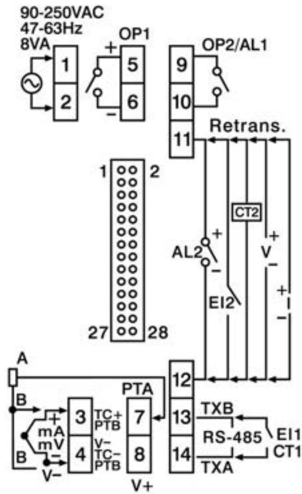
2-23 R22 Terminal Connection
