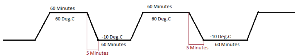
4-5 Temperature Profile for Temperature Cycling Chamber
