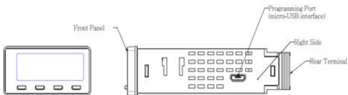
2-2 C22 Dimension without Clamp
