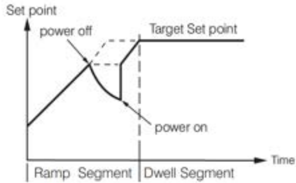
3-29 Power failure recovery from the profile at Ramp segment
