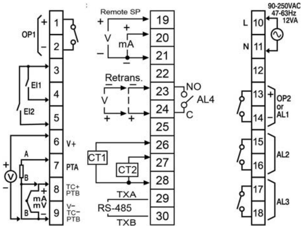
2-22 C72 Rear Terminal Connection
