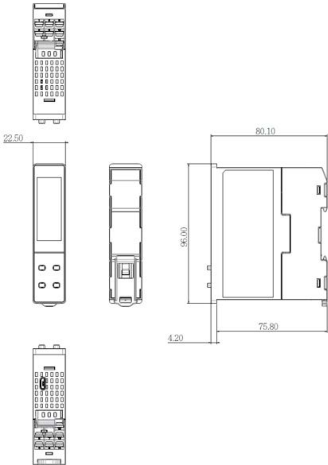
2-13 R22 Dimension
