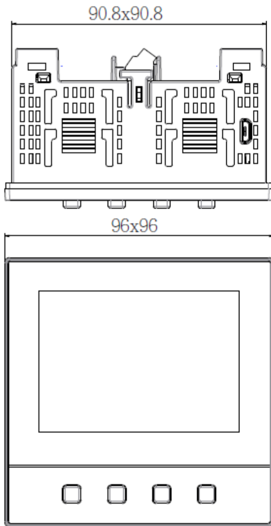
2-12 C42 Dimension without Clamp
