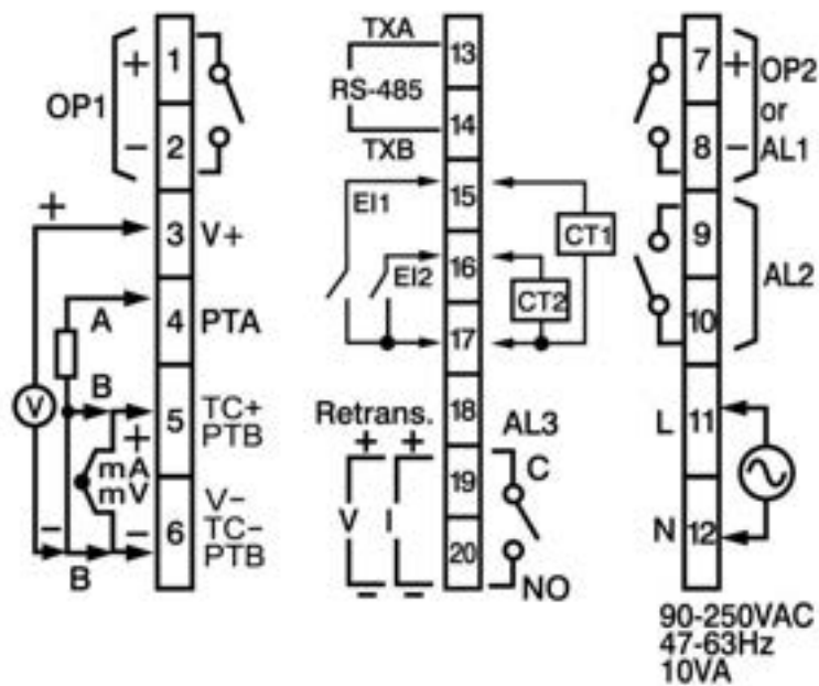
2-19 C62 Rear Terminal Connection
