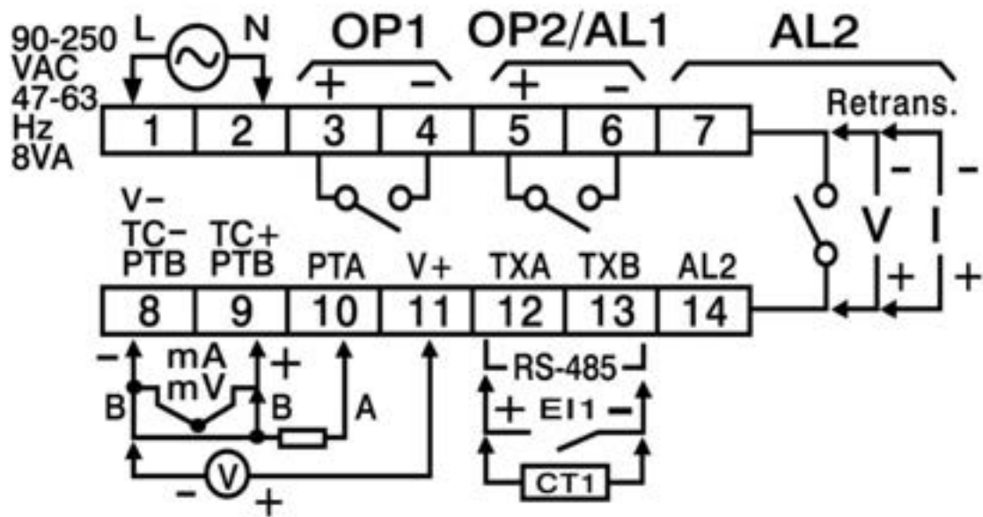
2-18 C22 Rear Terminal Connection
